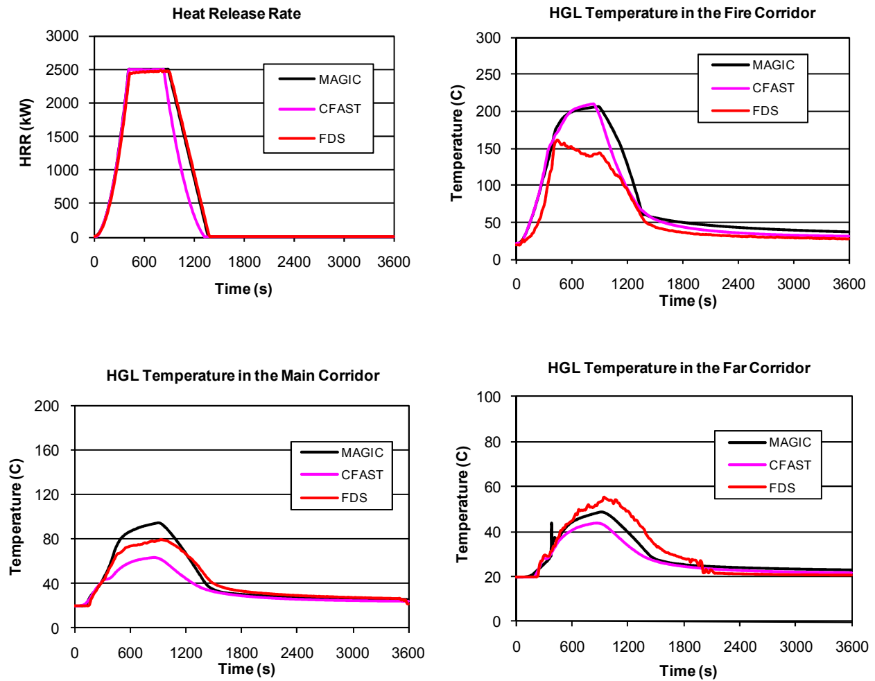
Figure G-5. Summary of modeling results for the Corridor scenario.
