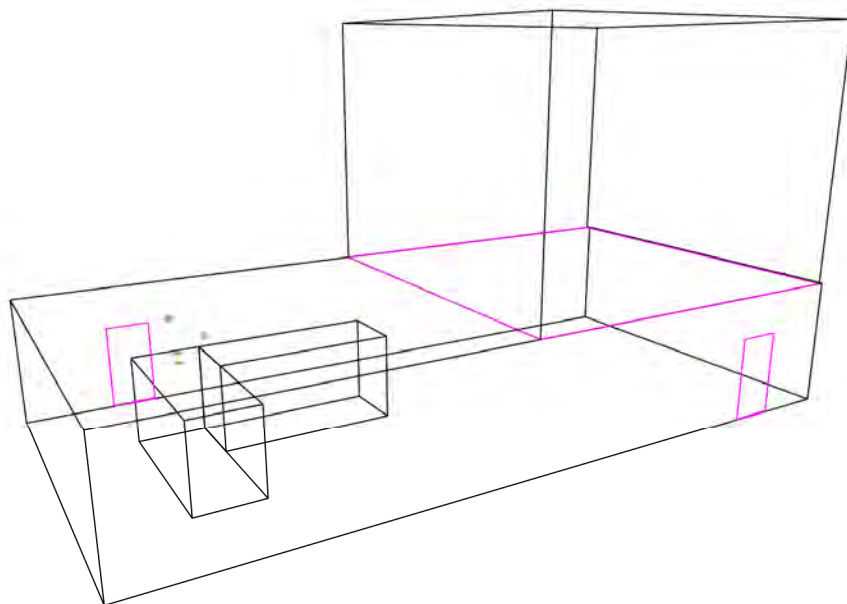
Figure D-4. Geometry two-height ceiling Switchgear Room as modeled in CFAST.
