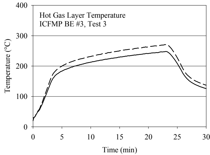
Figure 4-3. HGL Temperature as a function of time due to a 1000 kW fire (solid line) and an 1150 kW fire (dashed). Both predictions are by FDS. There is a 10 % increase in the temperature due to the 15 % increase in the HRR.
