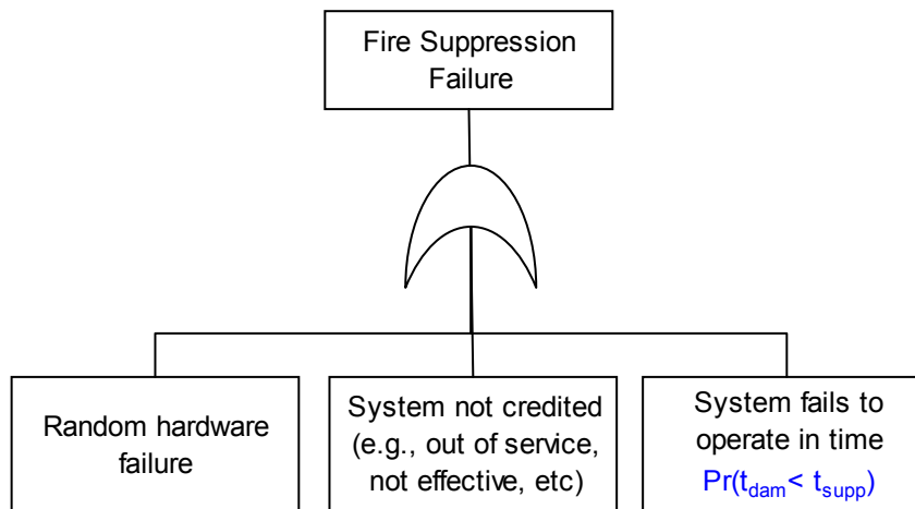
Figure 6-1. Generic fault tree depicting the logic for suppression failure
