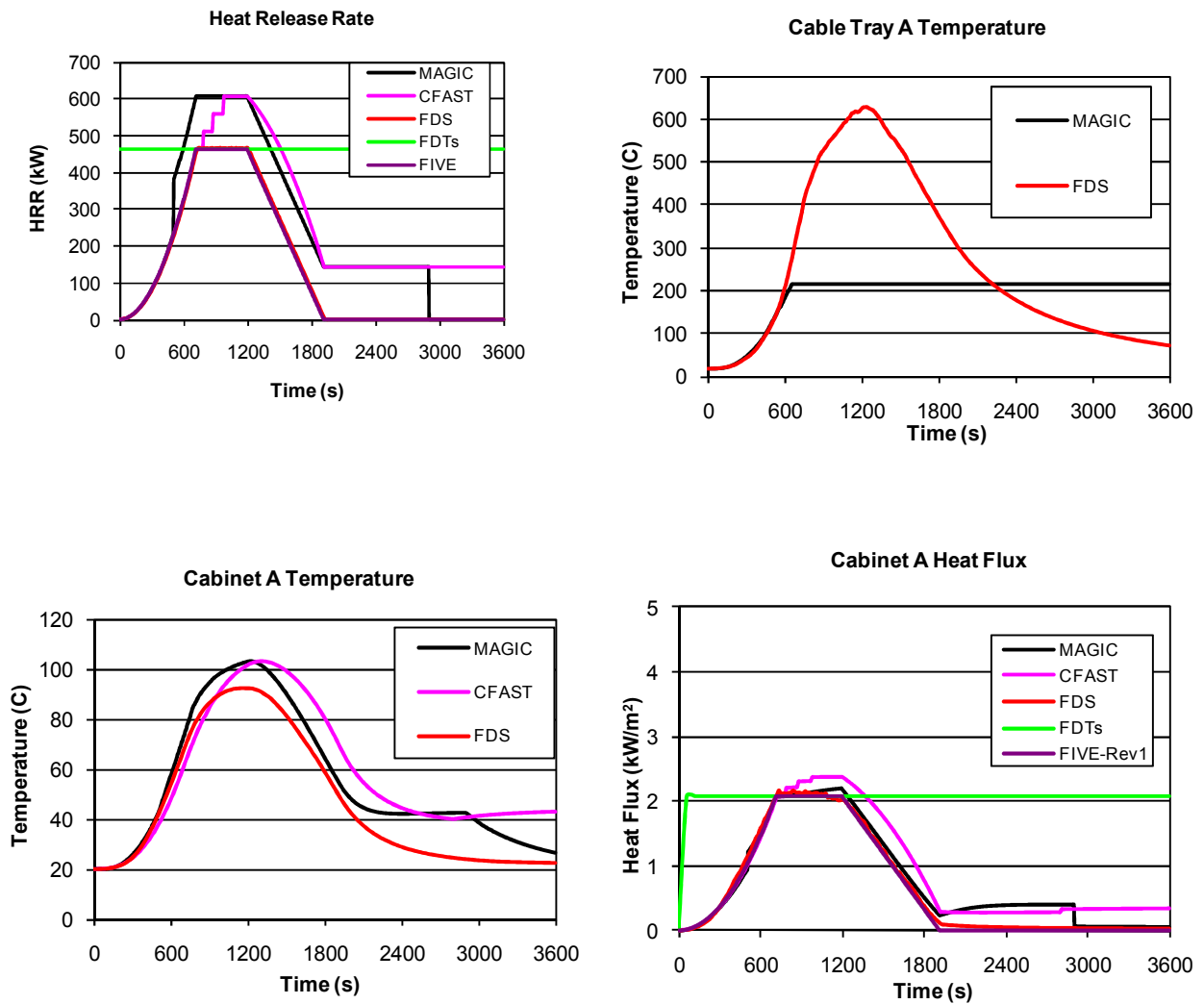
Figure B-3. Summary of simulation results for Switchgear Room cabinet fire.
