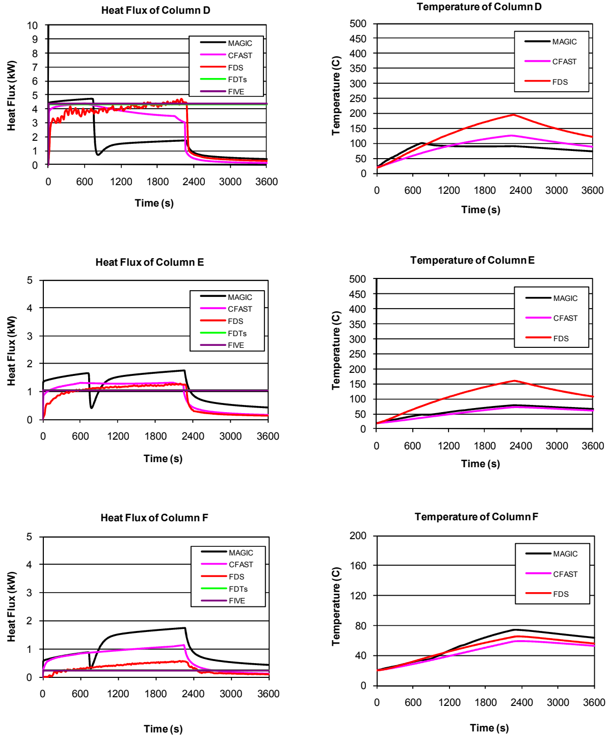
Figure F-5. Summary of simulation results for the Turbine Building.
