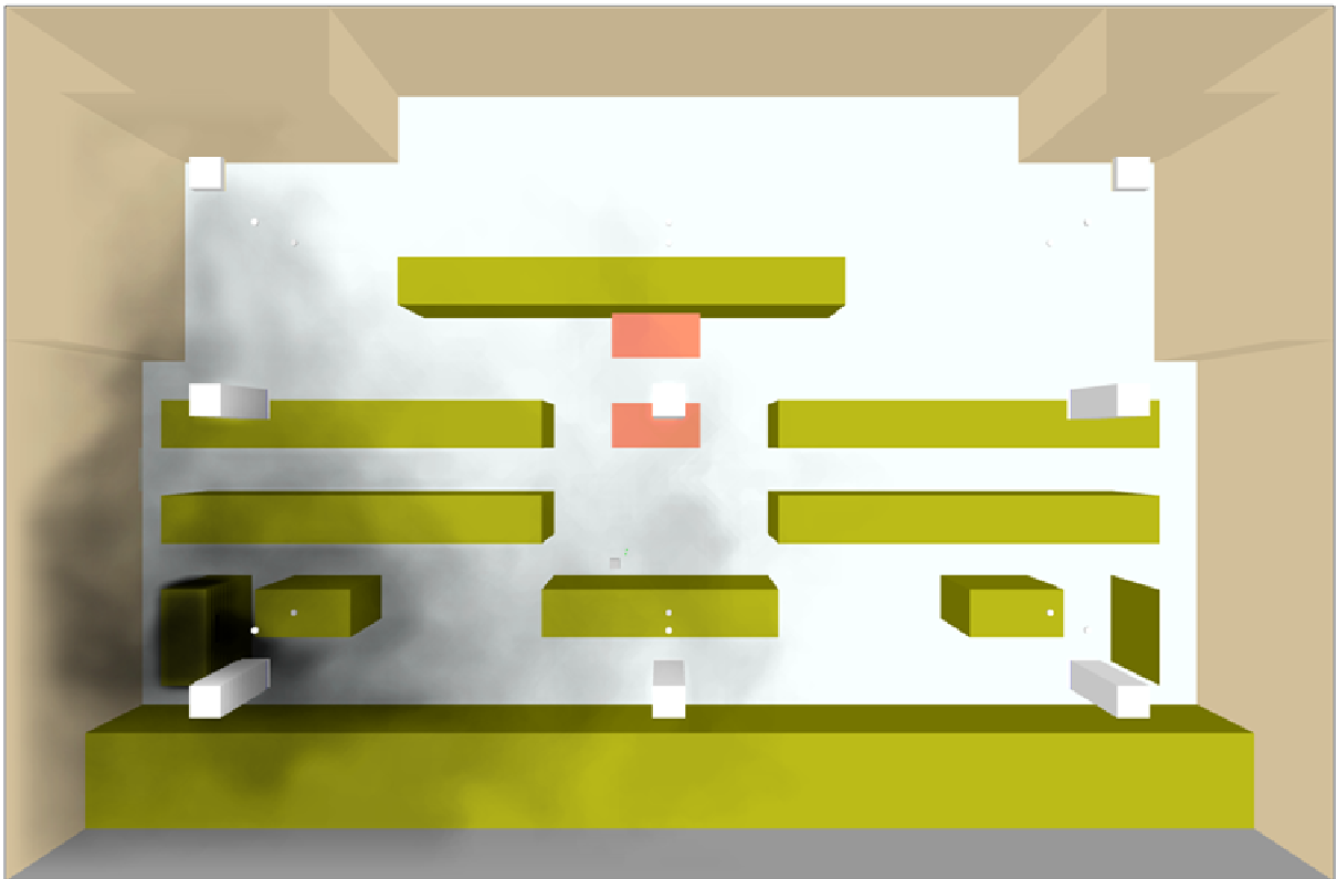
Figure A-5. FDS/Smokeview rendering of the Main Control Room, as seen from above.
