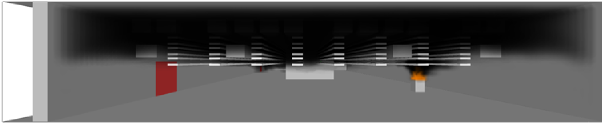
Figure E-4. FDS/Smokeview rendering of the Cable Spreading Room scenario.
