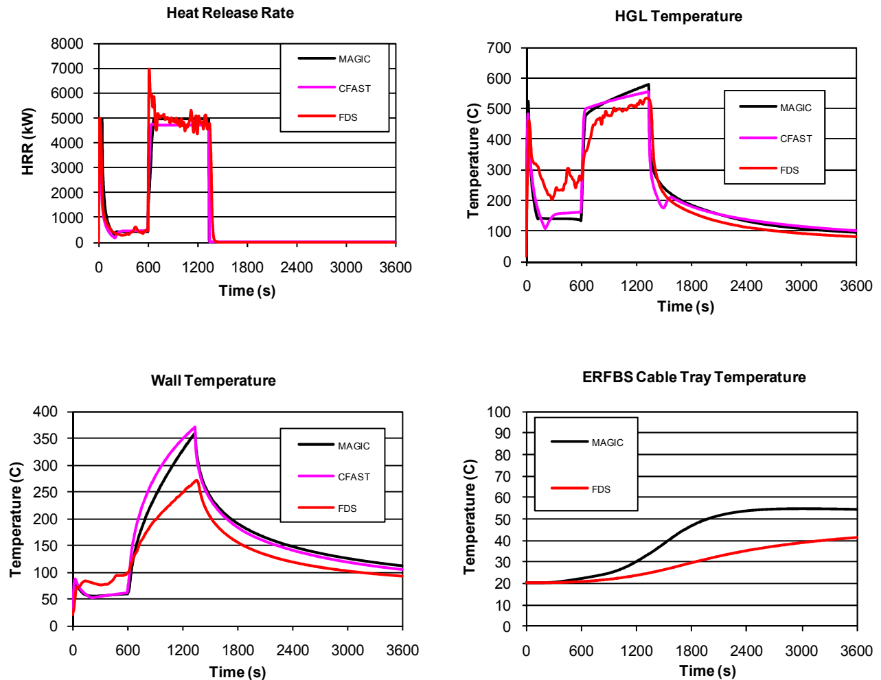
Figure C-3. Summary of results for the Pump Room fire scenario.
