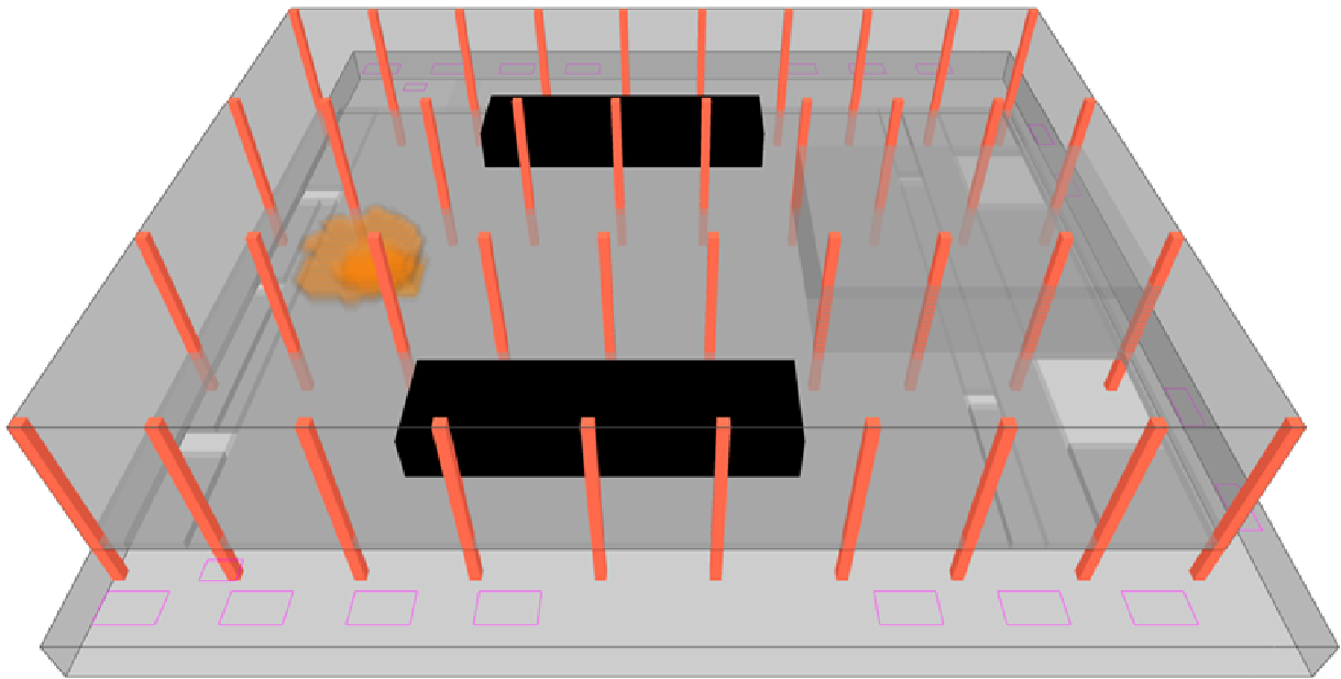
Figure F-4. FDS/Smokeview rendering of the Turbine Building scenario.
