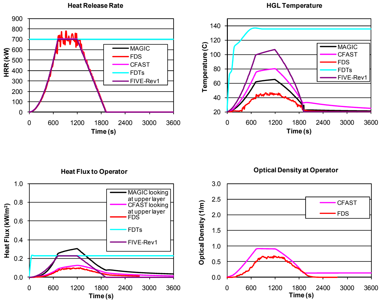
Figure A-6. Summary of the simulation results for the Main Control Room.
