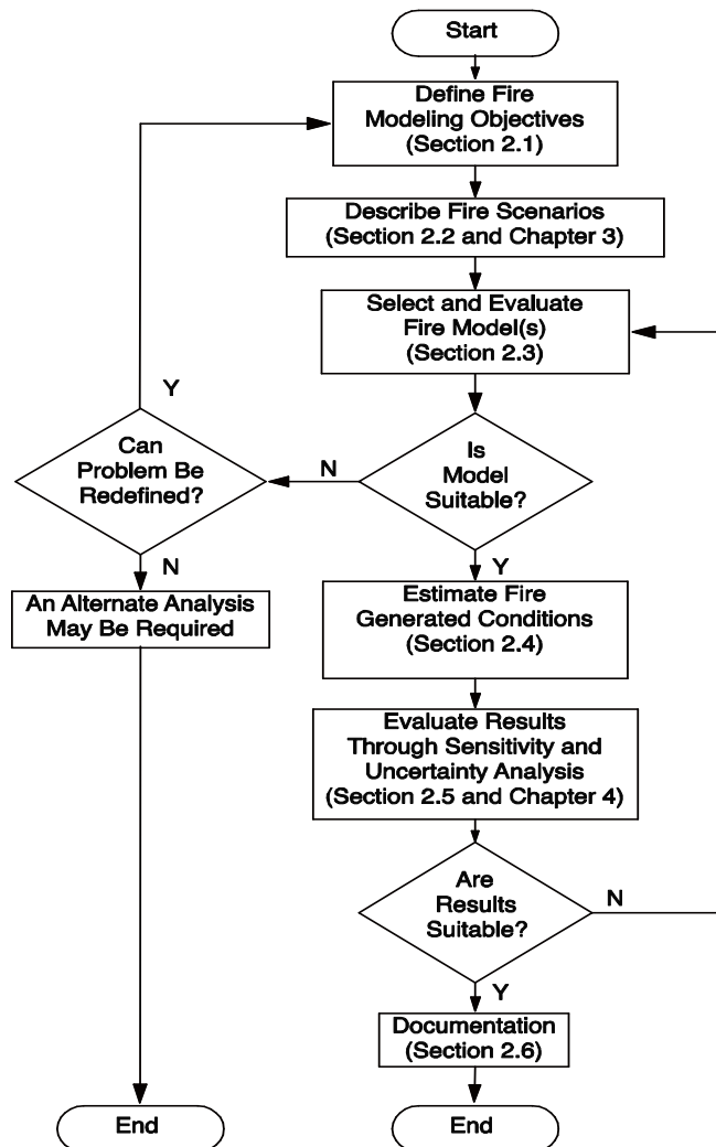
Figure 2-1. Fire Modeling Process
