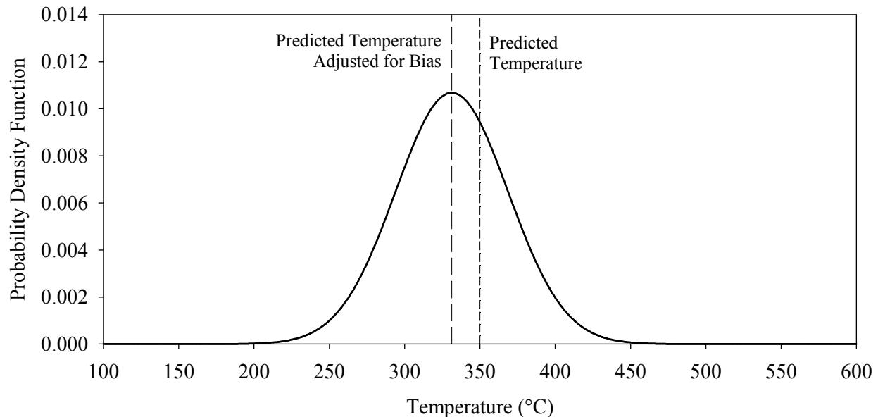
Figure 4-2. Normal distribution of the “true” value of the HGL Temperature of a postulated fire scenario
