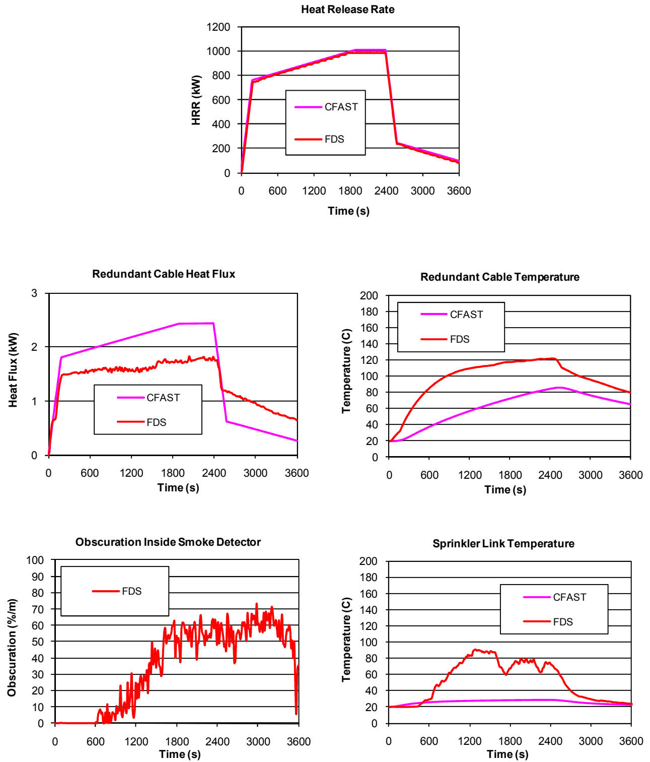
Figure H-4. Summary of simulation results for the Annulus.
