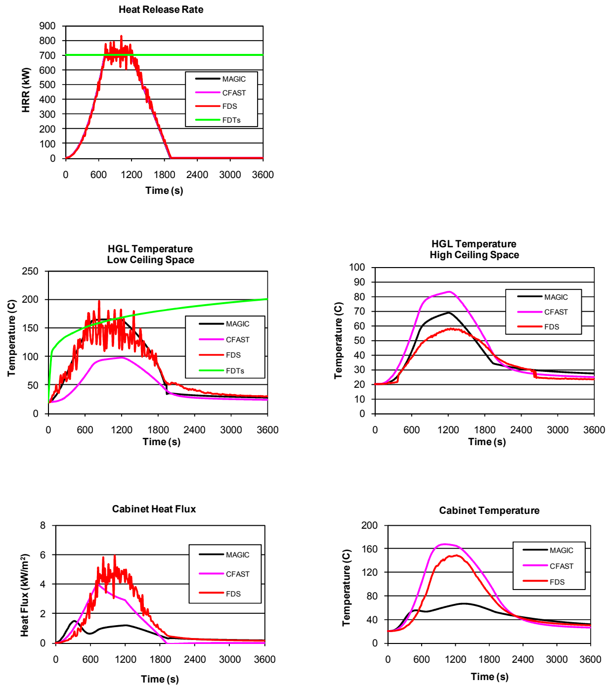
Figure D-6. Summary of simulation results for the MCC/Switchgear Room.
