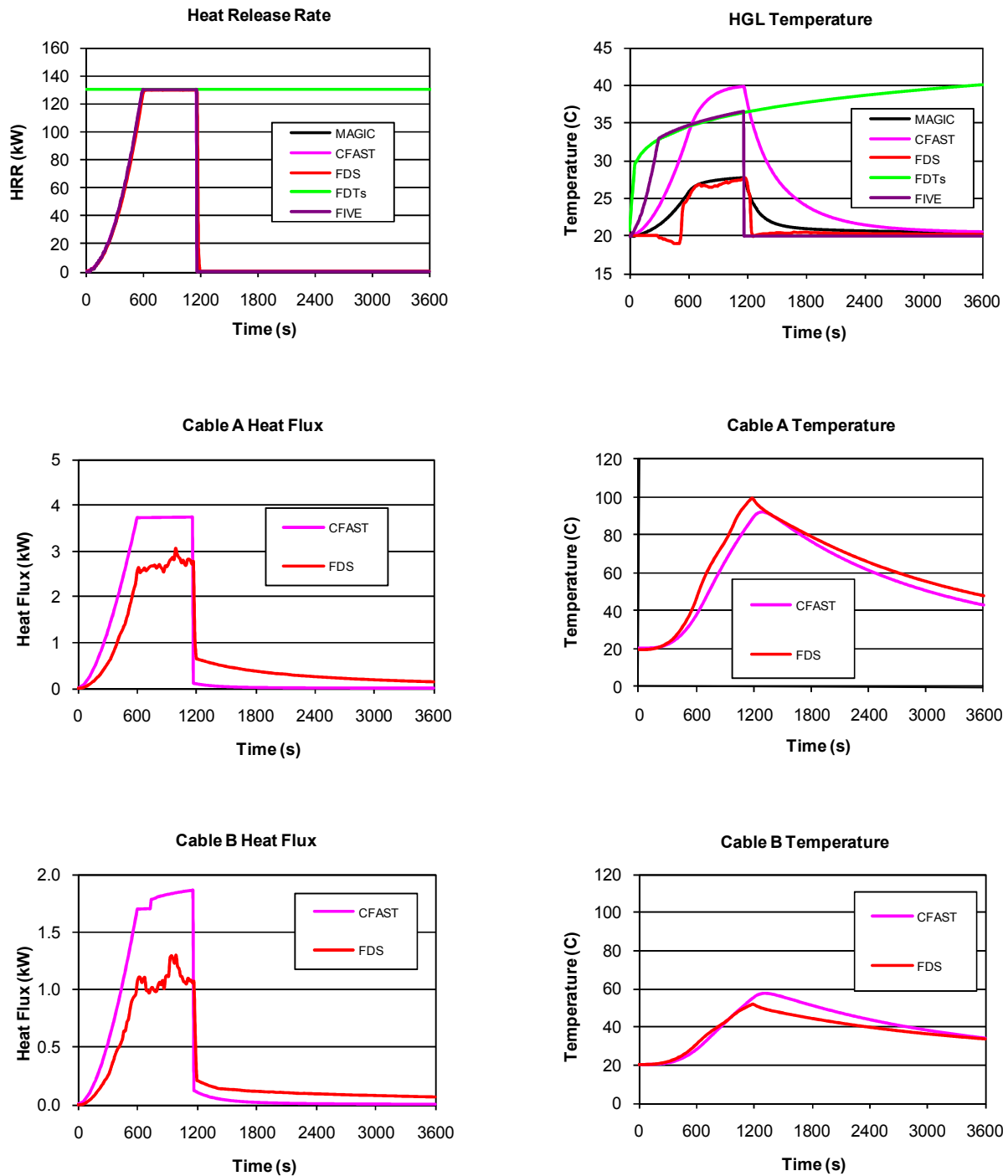
Figure E-5. Summary of simulation results for the Cable Spreading Room.
