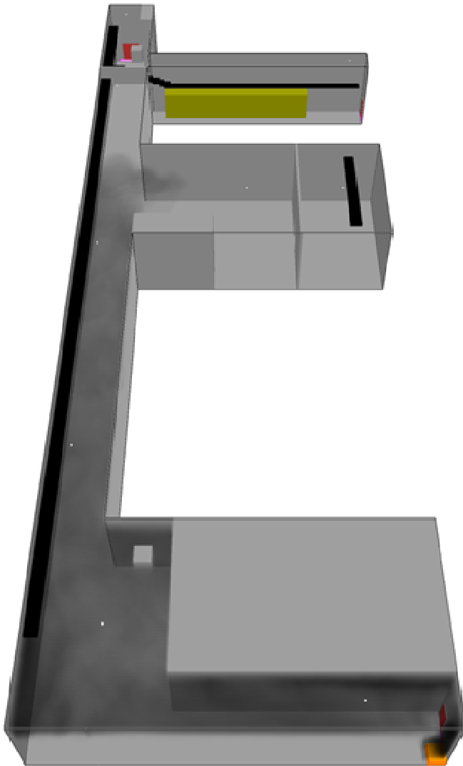
Figure G-4. FDS/Smokeview rendering of the Corridor scenario.
