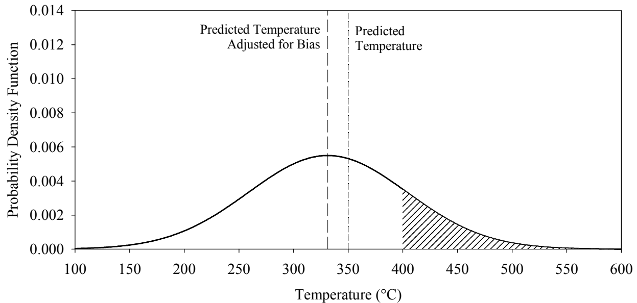
Figure 4-4. Normal distribution of the “true” value of the HGL Temperature of a postulated fire scenario. The shaded area represents the probability that the temperature exceeds 400 °C.
