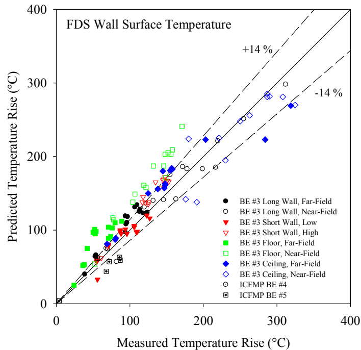
Figure 4-1. Sample plot from NUREG-1824.
