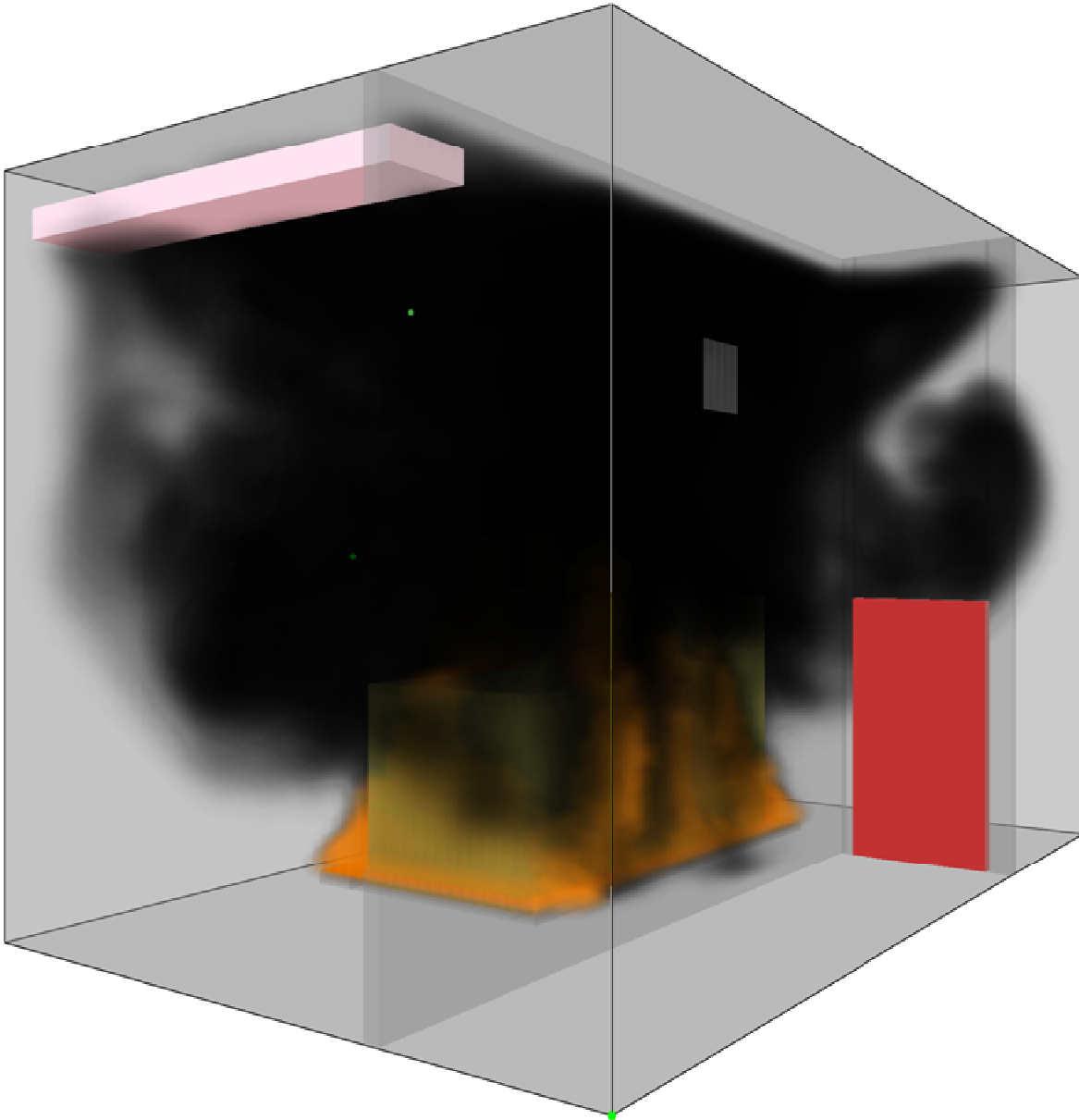
Figure C-2. FDS/Smokeview rendering of the Pump Room scenario at the early stage of the fire, before the compartment becomes under-ventilated.
